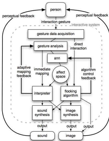
Figure 3. Structure of the interactive system in Codespace .
